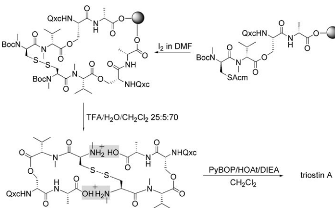
Scheme 2. Dimerization and cyclization to obtain triostin A.
