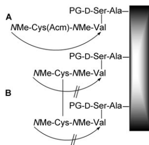
Figure 3. Protection by conformationally restricted mobility prevents DKP formation.
