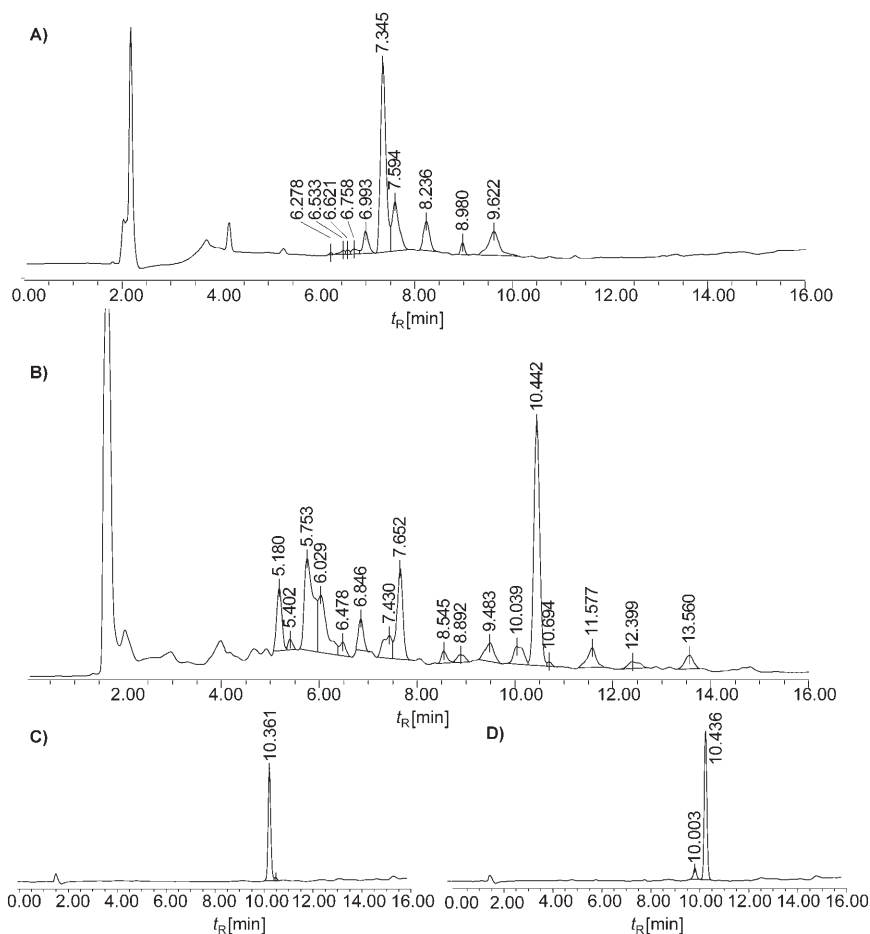
Figure 4. Analytical HPLC of A) crude dimer ( t_R = 7.34 min), B) crude triostin A ( t_R = 10.44 min), C) most polar and D) least polar conformer.
