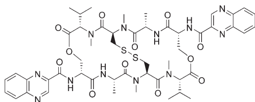
Figure 1. Structure of triostin A.
