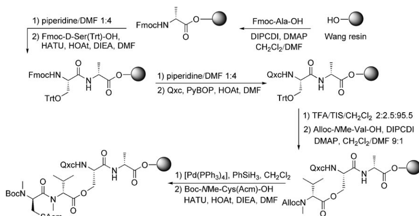
Scheme 1. Synthesis of the tetradepsipeptide of triostin A on solid-phase. HATU = O -(7-azabenzotriazol-1-yl)tetramethyluronium hexafluorophosphate; DIPCDI = N,N' -diisopropylcarbodiimide; Qxc = 2-quinoxaline carboxylic unit; PyBOP = benzotriazol-1-yloxy-tris (dimethylamino) phosphonium hexafluorophosphate; HOAt = 1-hydroxy-7-azabenzotriazole.
